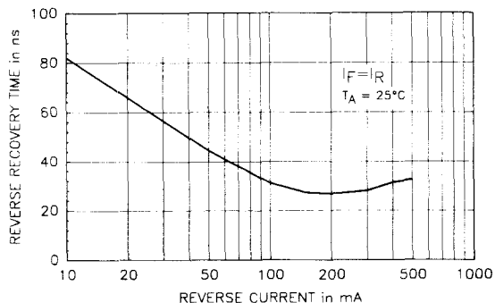
REVERSE RECOVERY TIME vs REVERSE CURRENT
