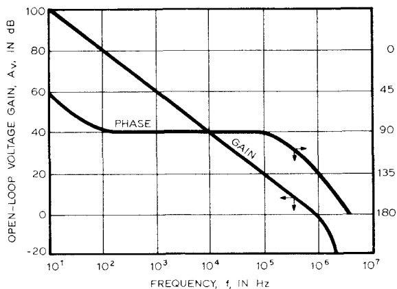
OPEN-LOOP VOLTAGE GAIN AND PHASE AS A FUNCTION OF FREQUENCY
