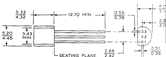
Dimensions in Millimeters (Based on 1" = 25.4 mm)
