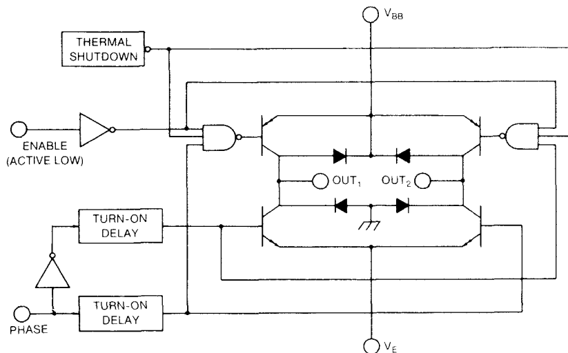
FUNCTIONAL BLOCK DIAGRAM (ONE OF TWO DRIVERS)
