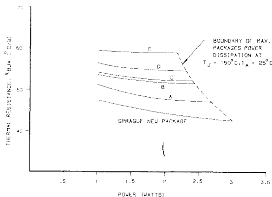
FIGURE 15 Thermal resistance versus power dissipation capability for various packages.
