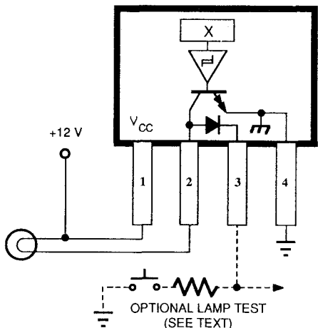
FIGURE 3 TYPICAL LAMP DRIVER APPLICATION
