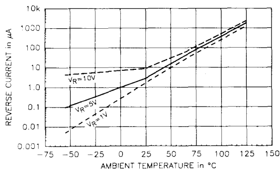
REVERSE CURRENT vs TEMPERATURE
