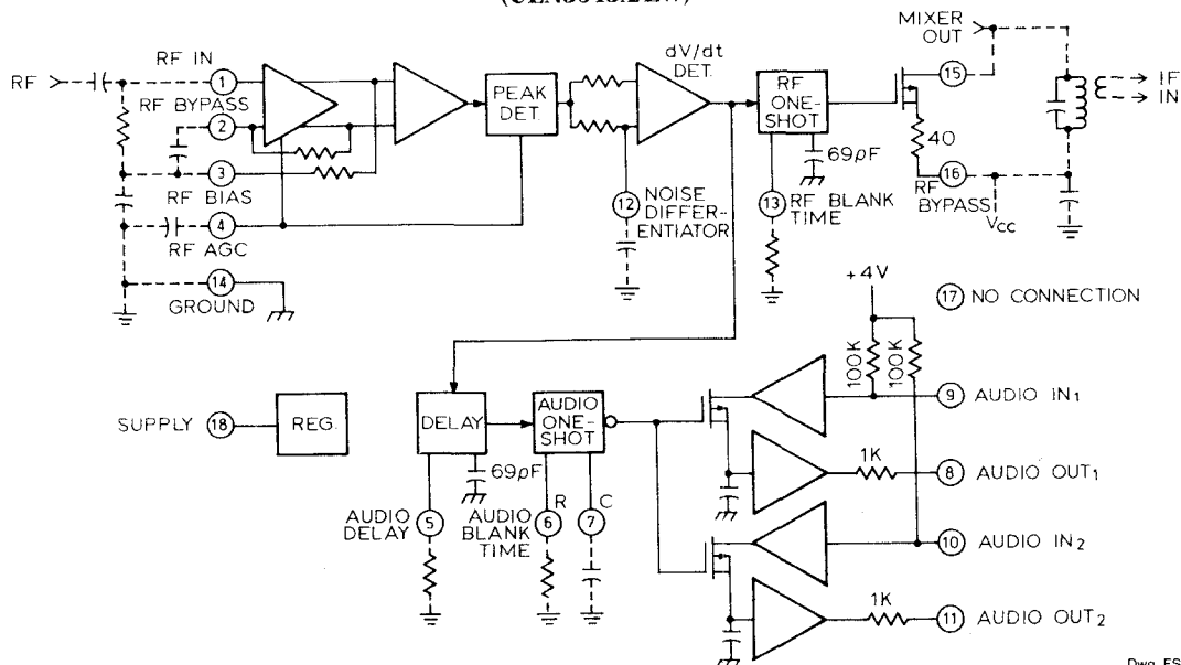
FUNCTIONAL BLOCK DIAGRAM (ULN3845A/LW)
