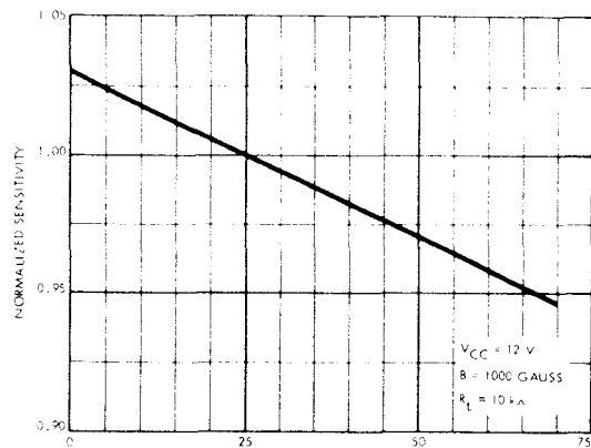
NORMALIZED SENSITIVITY AS A FUNCTION OF TEMPERATURE
