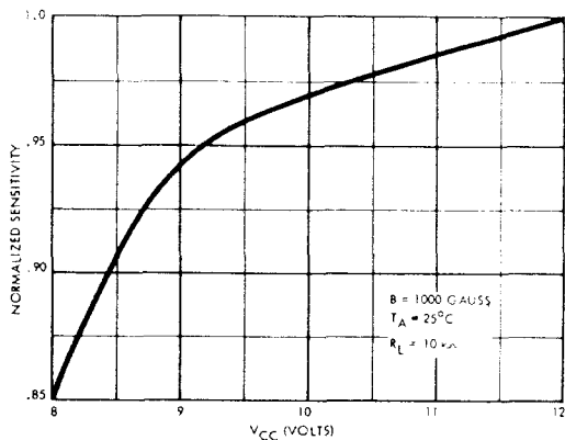
NORMALIZED SENSITIVITY AS A FUNCTION OF V_{CC}
