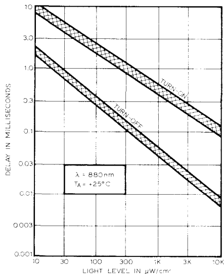
PROPAGATION DELAY AS A FUNCTION OF ILLUMINANCE
