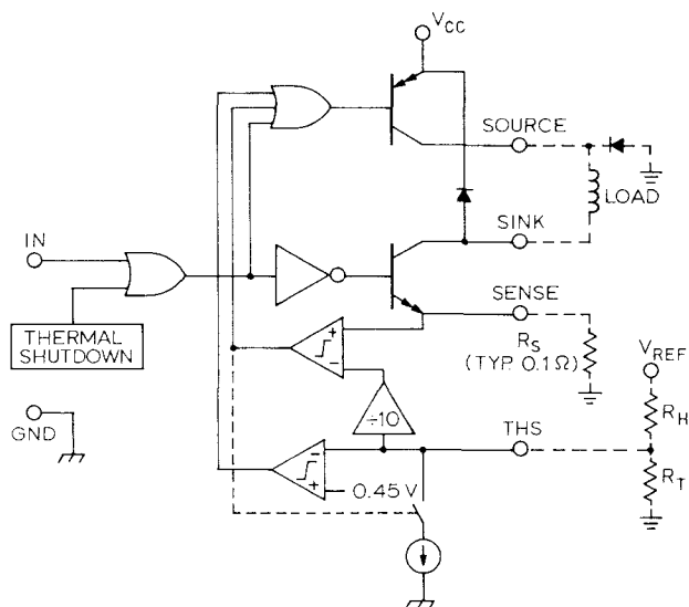
FUNCTIONAL BLOCK DIAGRAM (ONE OF TWO DRIVERS)
