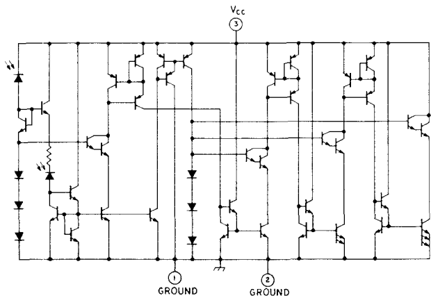
SCHEMATIC
