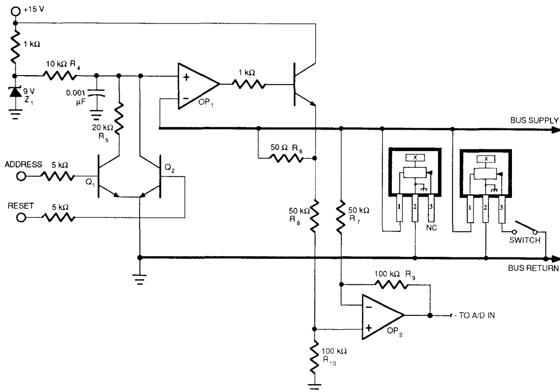
FIGURE 5 BUS INTERFACE SCHEMATIC
