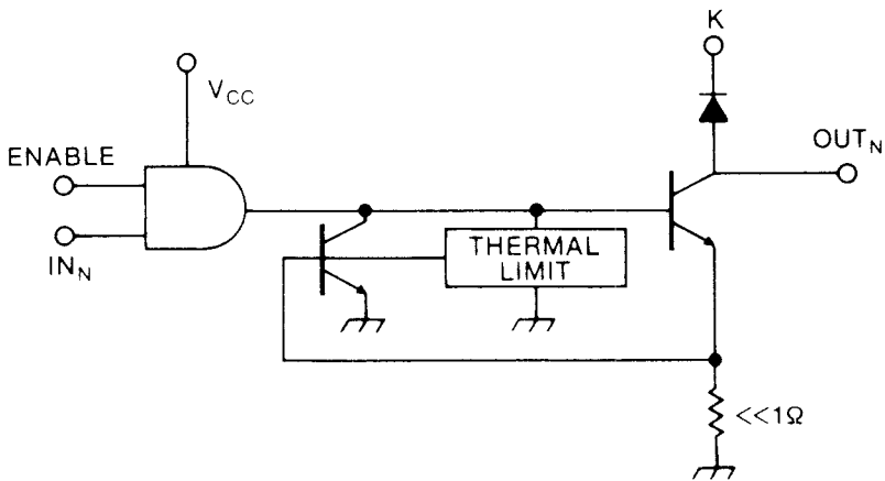
(1 OF 4 CHANNELS)
