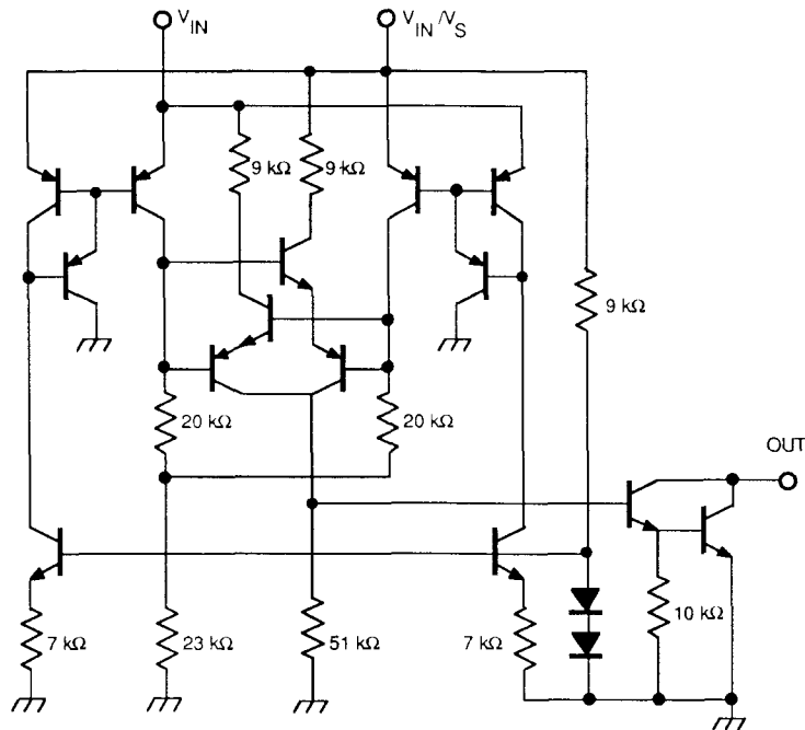
SIMPLIFIED SCHEMATIC (SINGLE DIFFERENTIAL SENSE AMPLIFIER)
