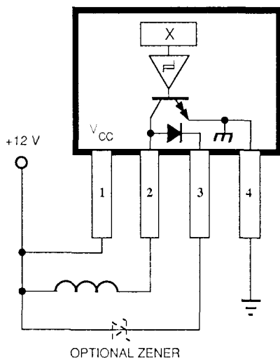
FIGURE 6 TYPICAL RELAY/SOLENOID DRIVER APPLICATION
