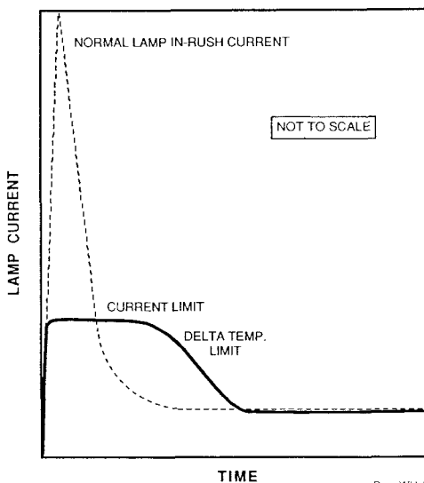
FIGURE 4 LAMP CURRENT vs TIME
