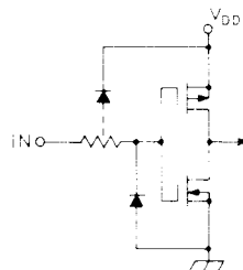
TYPICAL INPUT CIRCUIT
