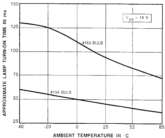
FIGURE 5 LAMP TURN-ON TIME
