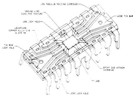
FIGURE 14 New web 16-lead PDIP.
