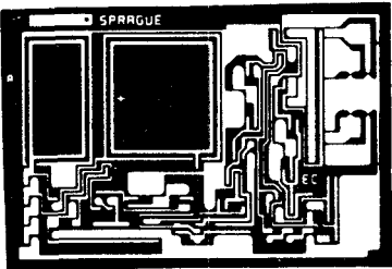
UNPACKAGED CHIP
