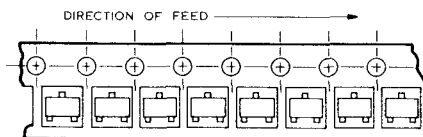
MECHANICAL ORIENTATION *
