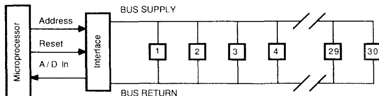
FIGURE 4 BUS INTERCONNECTION
