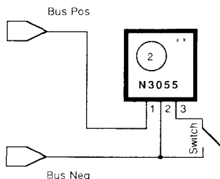
FIGURE 3 MECHANICALLY ACTUATED SENSOR
