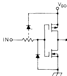
TYPICAL INPUT CIRCUIT
