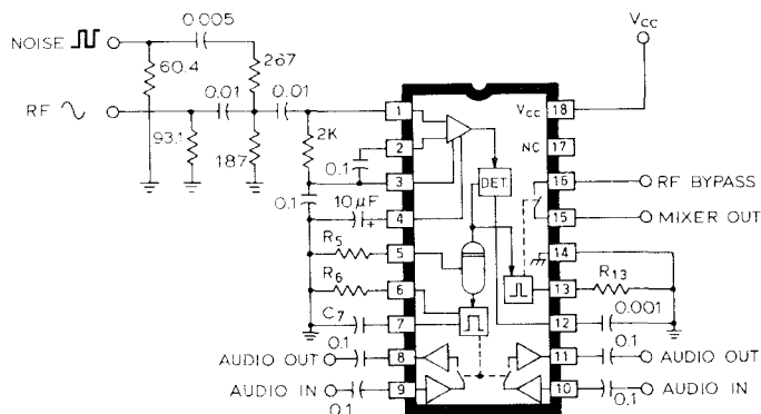
TEST CIRCUIT FIGURE 1
