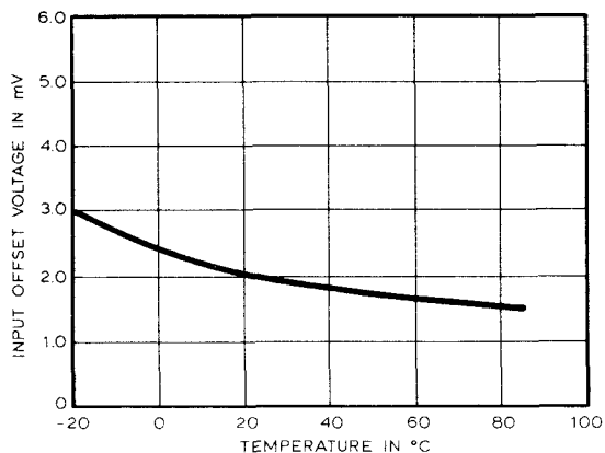
INPUT OFFSET VOLTAGE AS A FUNCTION OF TEMPERATURE
